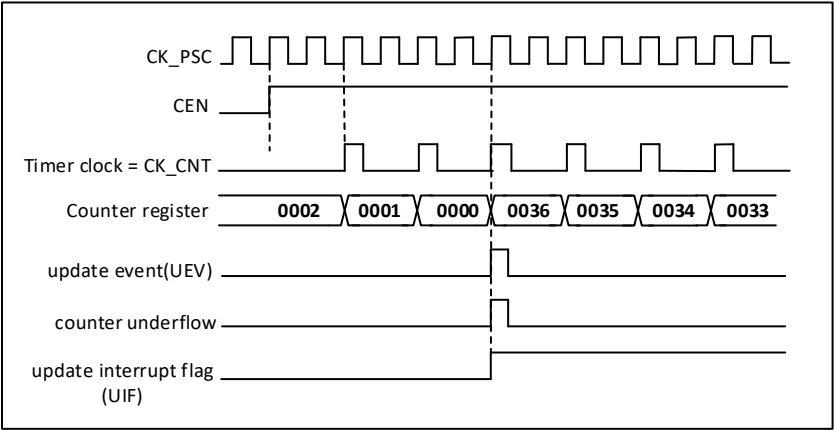
Figure 17-11 Counter timing diagram, internal clock divided by 2
