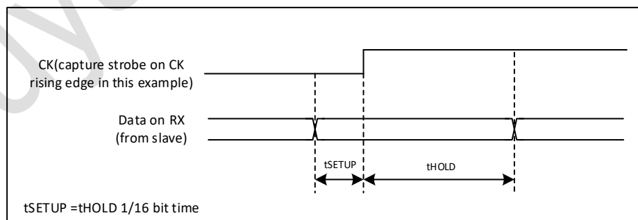
Figure 25-12 RX data sample/hold time
