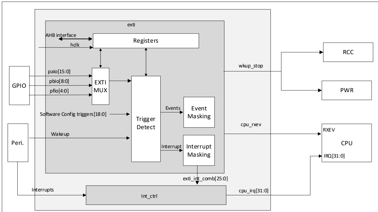
Figure 12-1 EXTI diagram
