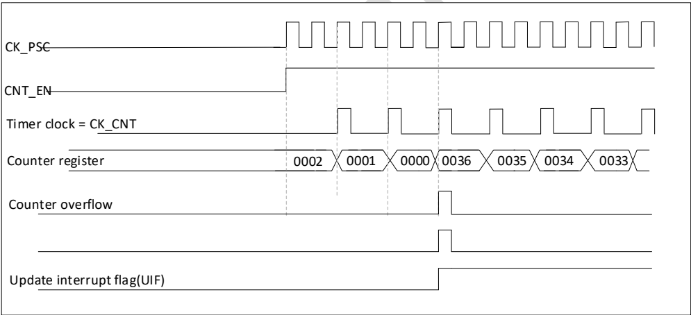
Figure 16-16 Counter timing diagram, internal clock divided by 2, TIMx_ARR = 0x36
