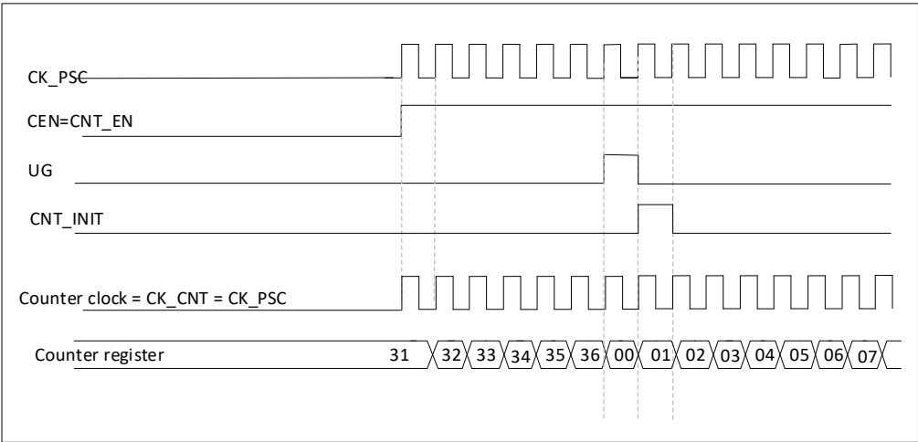
Figure 16-22 Control circuit in normal mode, internal clock divided by 1
