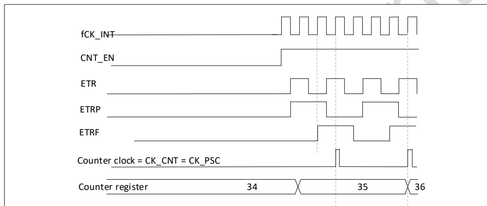
Figure 16-26 Control circuit in external clock mode 2
