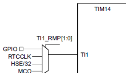
Figure 8-2 Frequency measurement with TIM14 in capture mode
