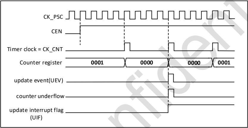
Figure 17-12 Counter timing diagram, internal clock divided by 4
