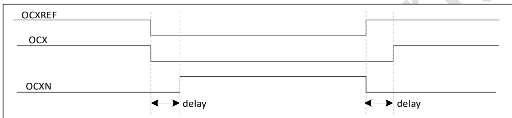
Figure 16-37 Complementary output with dead-time insertion
