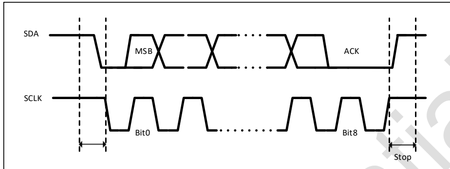
Figure 24-2 I2C bus protocol
