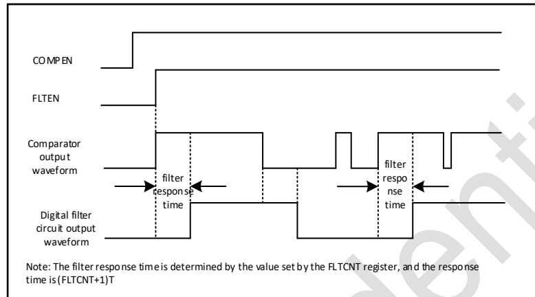
Figure 15-3 COMP filter
