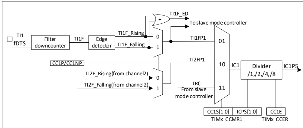
Figure 19-12 Capture/compare channel (example: channel 1 input stage)
