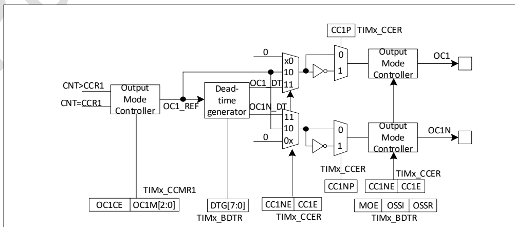
Figure 19-13 Capture/compare channel 1 main circuit
