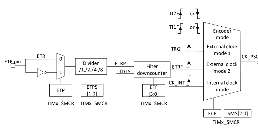
Figure 16-25 External trigger input block
