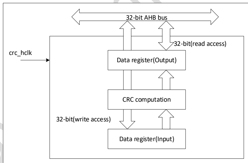
Figure 13-1 CRC calculation unit block diagram
